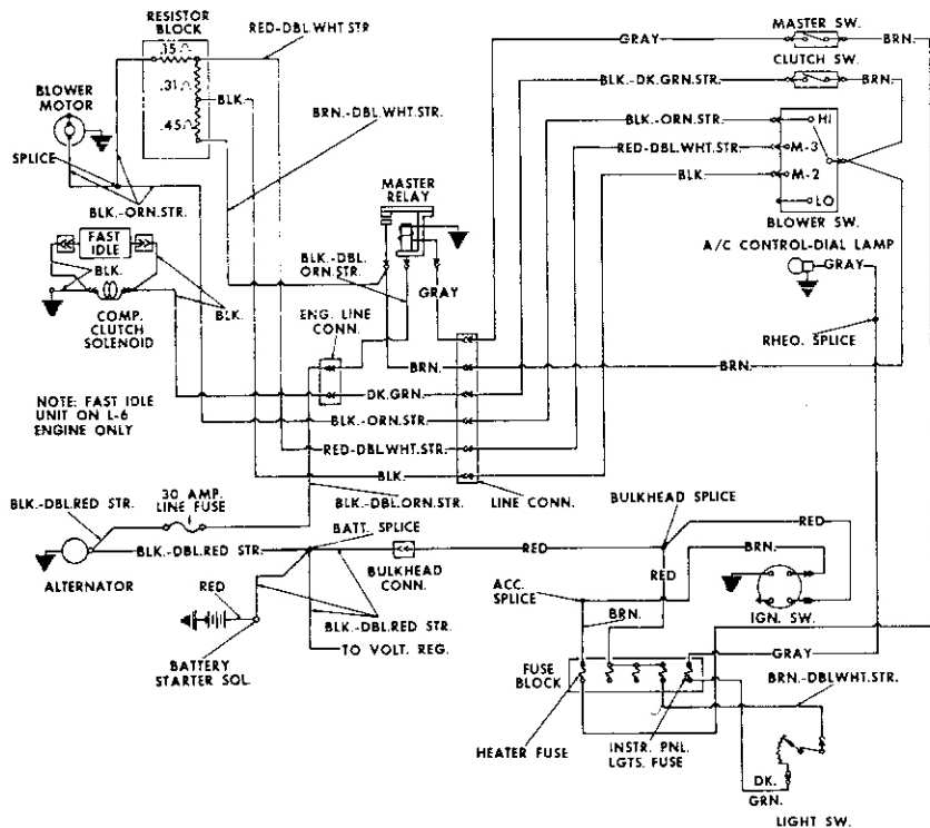
Air Conditioner . . 1965
