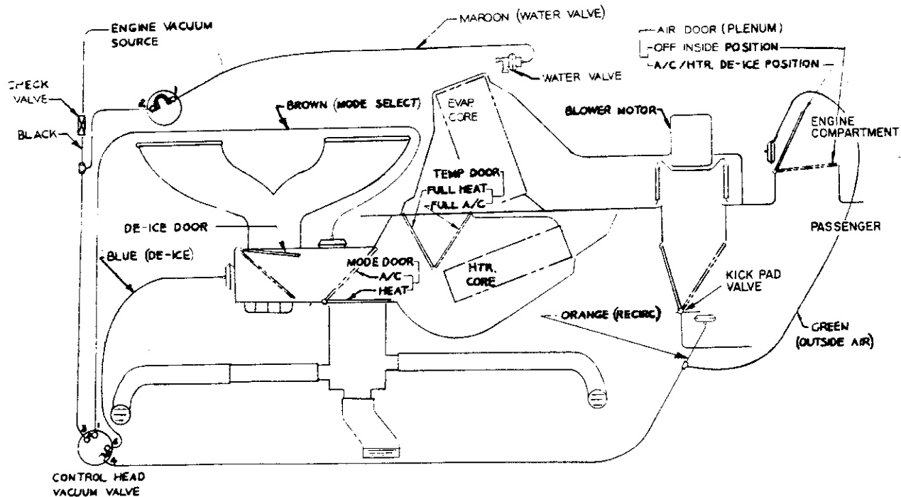
Air Conditioner Vacuum Circuit . . 1969 Tempest
