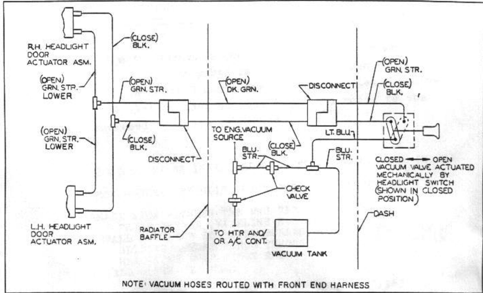
Fig. 12-41 Vacuum Operated Headlamp Door Schematic
