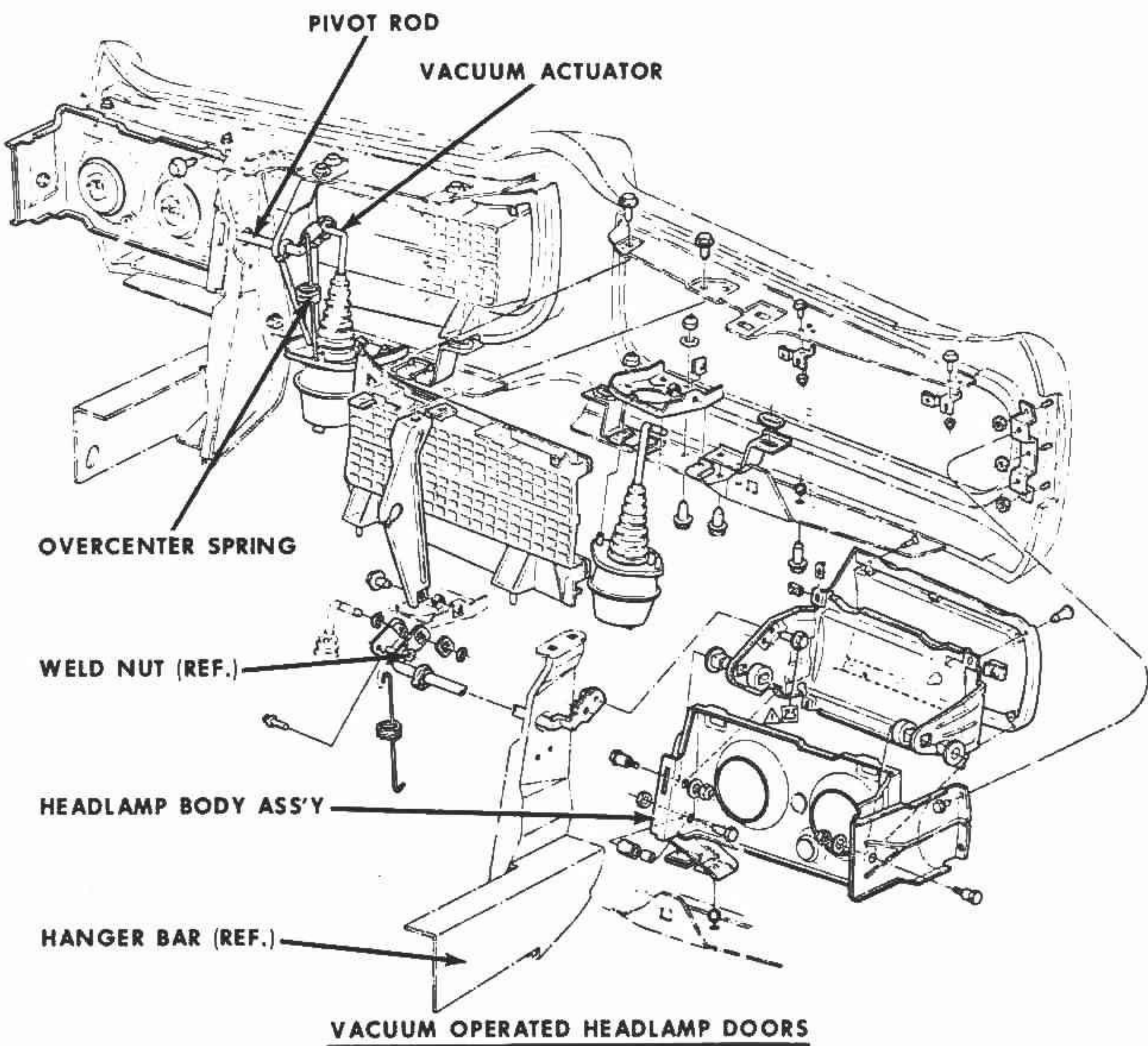
Fig. 12-40 Vacuum Operated Headlamp Doors—GTO
